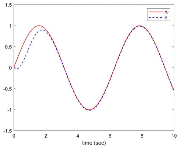
FIGURE 7 The responses of y_d and y of Example 2.
