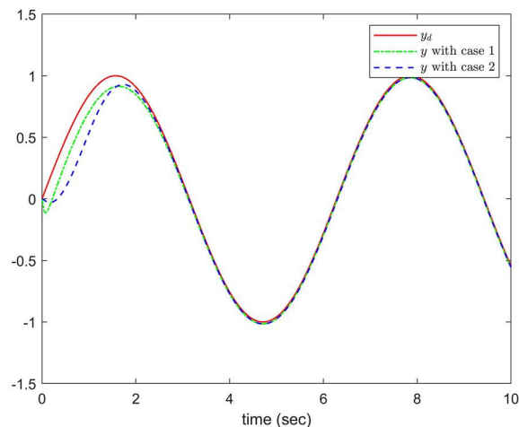
FIGURE 2 The responses of y_d and y of Example 1 in two cases.
