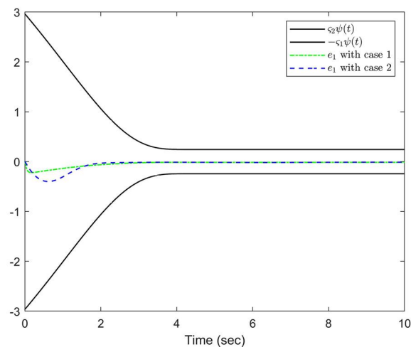
FIGURE 3 The responses of e_1 with performance constraint of Example 1 in two cases.
