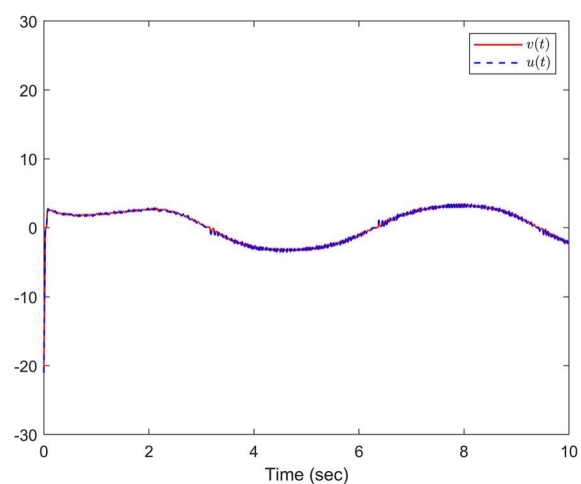
FIGURE 9 The responses of v(t) and u(t) of Example 2.
