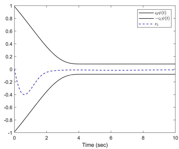
FIGURE 8 The response of e_1 with performance constraint of Example 2.
