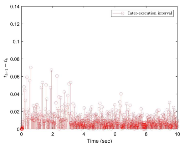
FIGURE 11 The response of inter-execution interval of Example 2.
