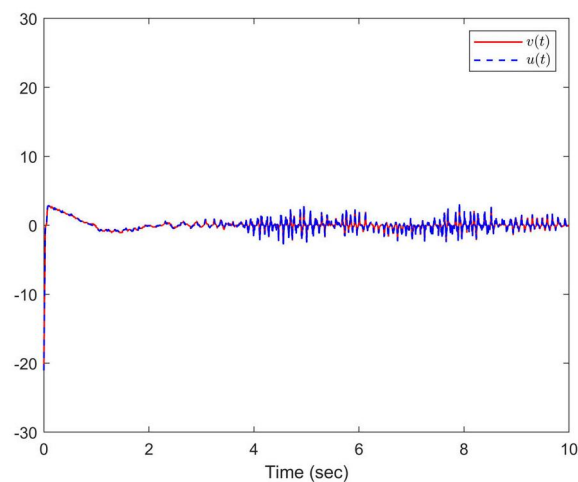
FIGURE 4 The responses of v(t) and u(t) of Example 1 in case 2.
