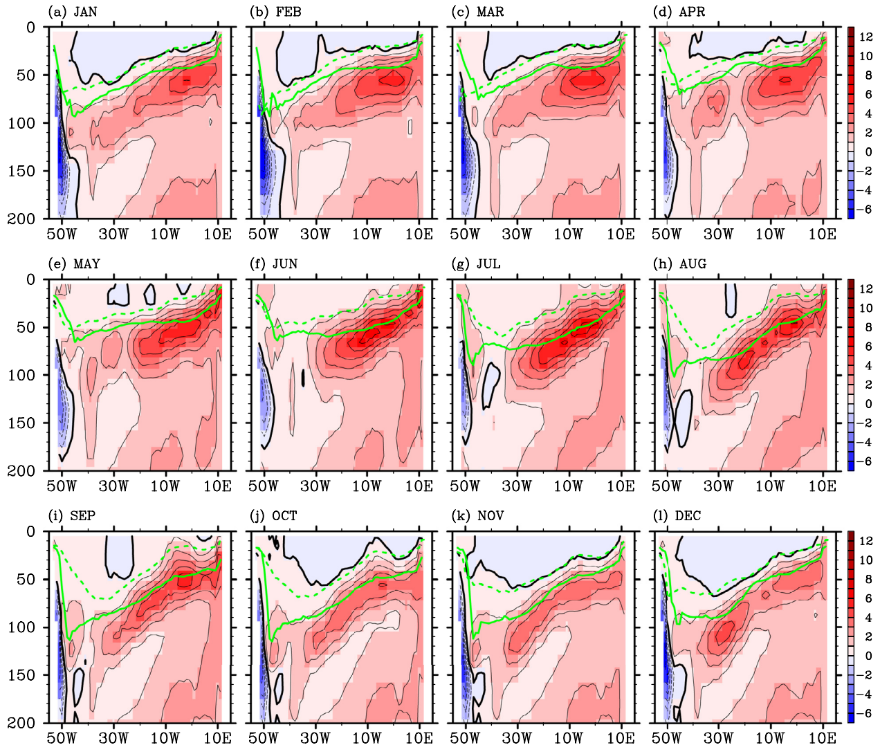
Fig. 8. Time-depth evolutions of the equatorial Atlantic temperature bias (shaded) and mixed layer depth (green solid line) averaged for 5°S–5°N obtained from EXP_OCN. The green dashed line is the mixed layer depth obtained from EN4. (For interpretation of the references to color in this figure legend, the reader is referred to the web version of this article.)
